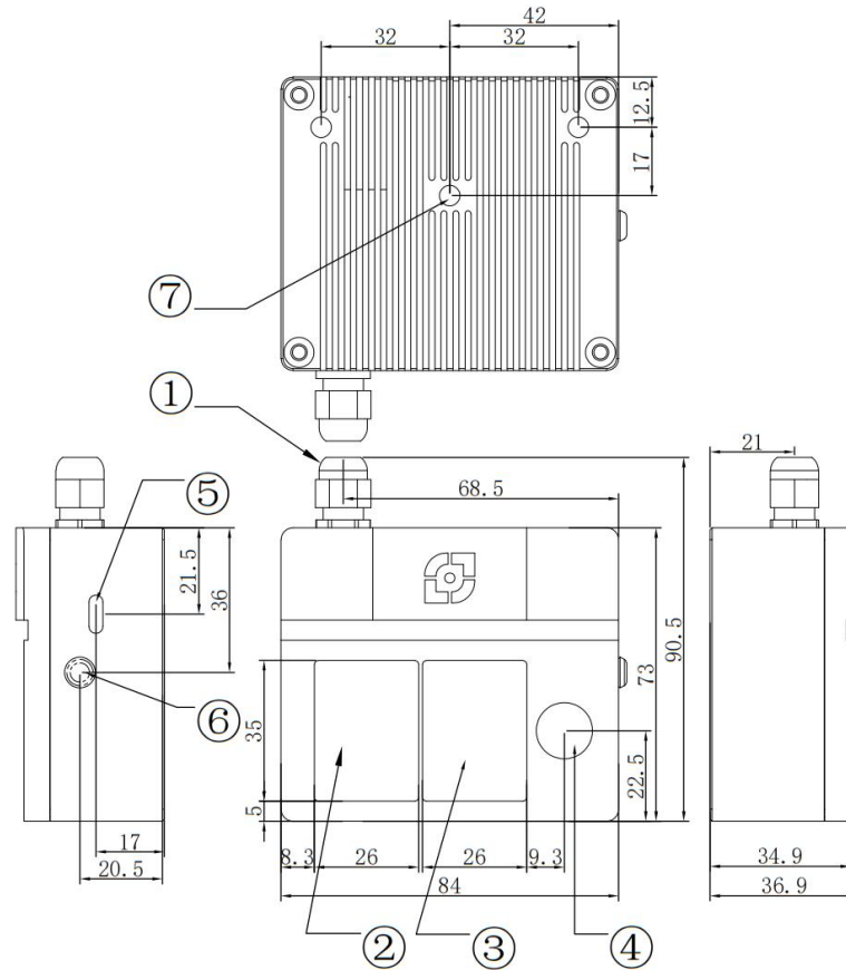
Figure 3. X-D1000 structure diagram
