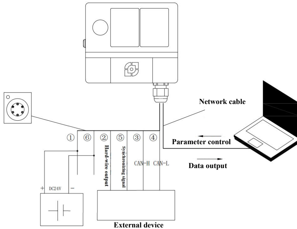
Figure 5. Product connection diagram
